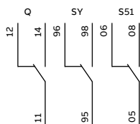
Auxiliary contacts Q (open/closed), SY (trip), S51 (trip unit tripping) and S52 (YO/YU tripping) status during sequences
